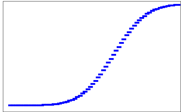
Figura 2.5 N(x, \sigma\sqrt{t})
