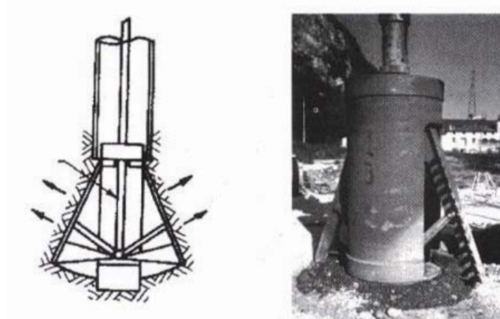
Fig. 1.3 Bote campana Ref. (2)
