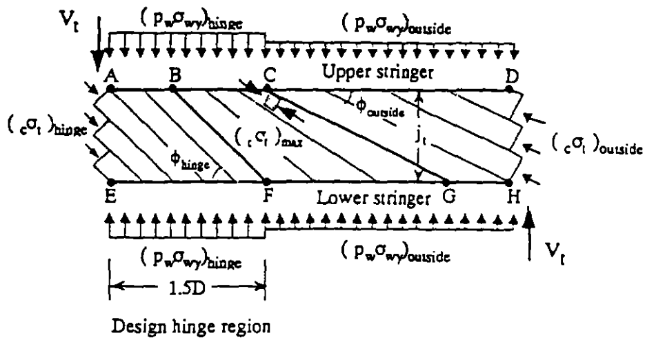
Fig. C6.11' Truss mechanism of a ductile member.
