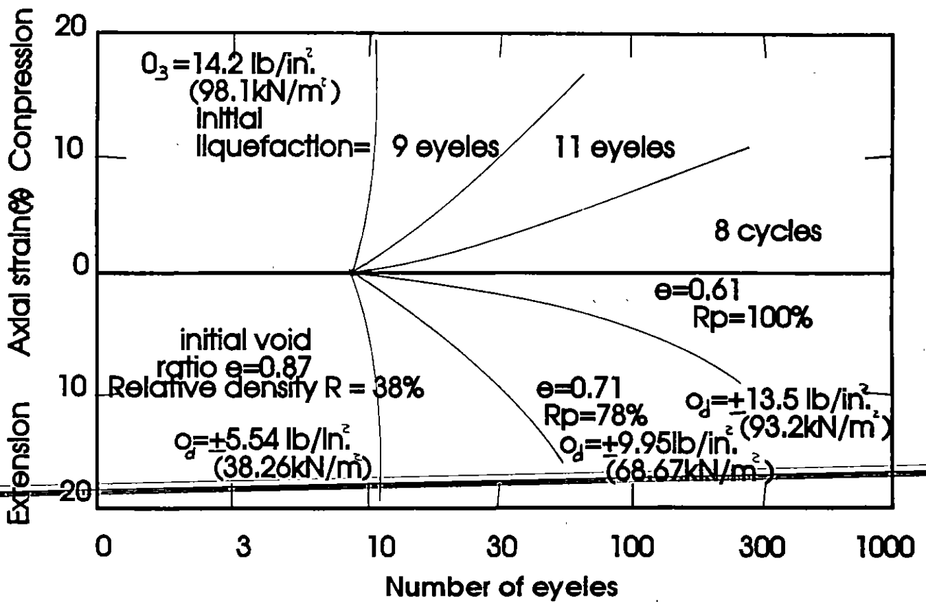
FIGURA 13 Axial strain after initial liquefaction for pulsatin load test at three densities for Sacramento River sand. (Seed, H. B., and Lee, K. L. (1966))
