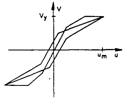
(c) Prestressed concrete
