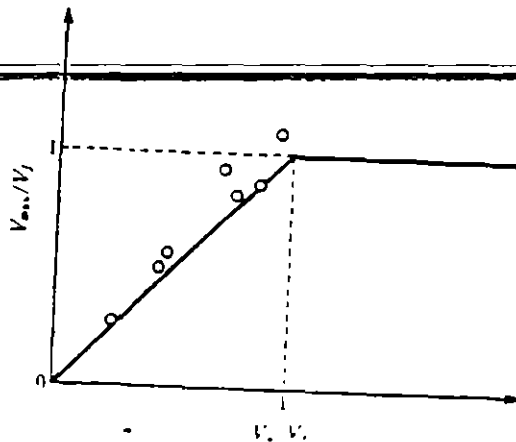
Fig. C6.27 Verification of strength equation.
