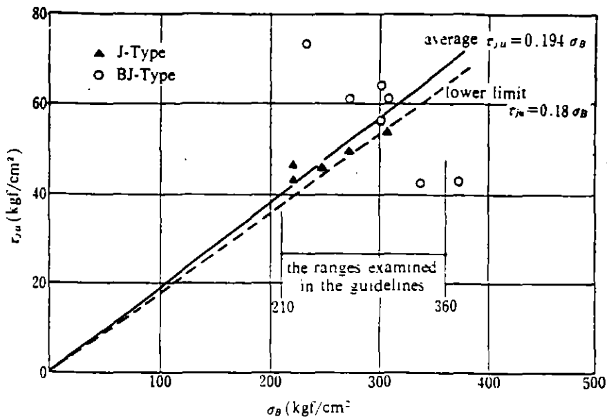
Fig. C 7.4 Average joint shear stress vs. compressive strength of concrete of exterior joint with a rotated T-shape subassemblage.
