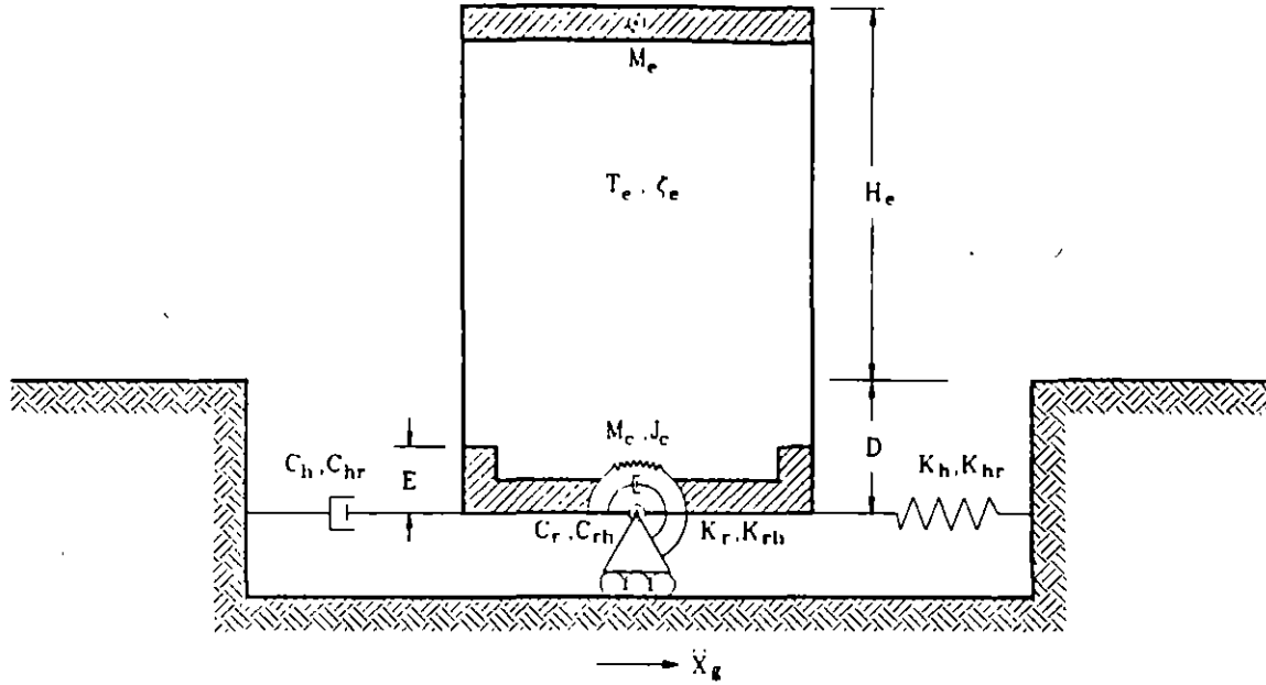
Fig. 2. Equivalent soil-structure system.
