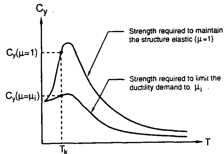
FIG. 1. Constant Displacement Ductility Nonlinear Response Spectra
