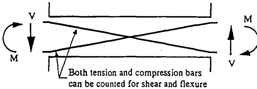
Fig. C6.15 X-shaped reinforcement placed diagonally across a member.
