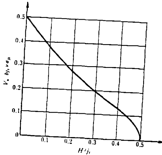
Fig. C6.26 Effect of the size of hole on the upper shear strength.
