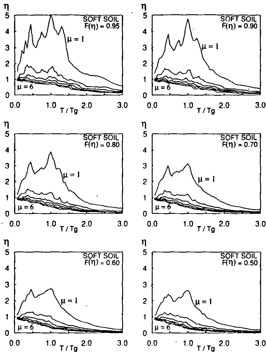
Figure 7. Probabilistic non-linear spectra of normalized strength demands for soft soil sites ( \mu = 1, 2, 3, 4, 5, 6 )
