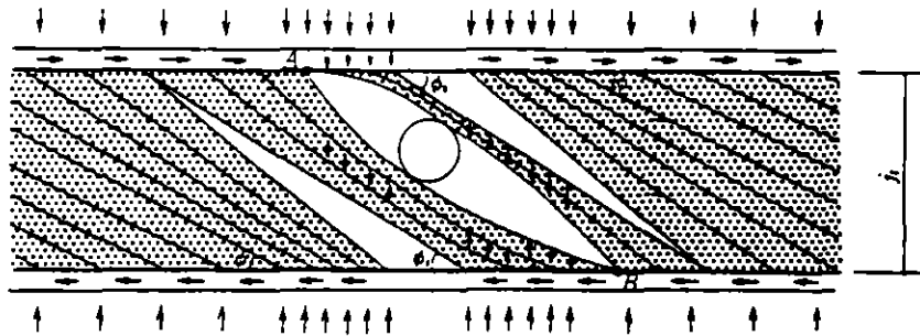
(b) Truss action.
