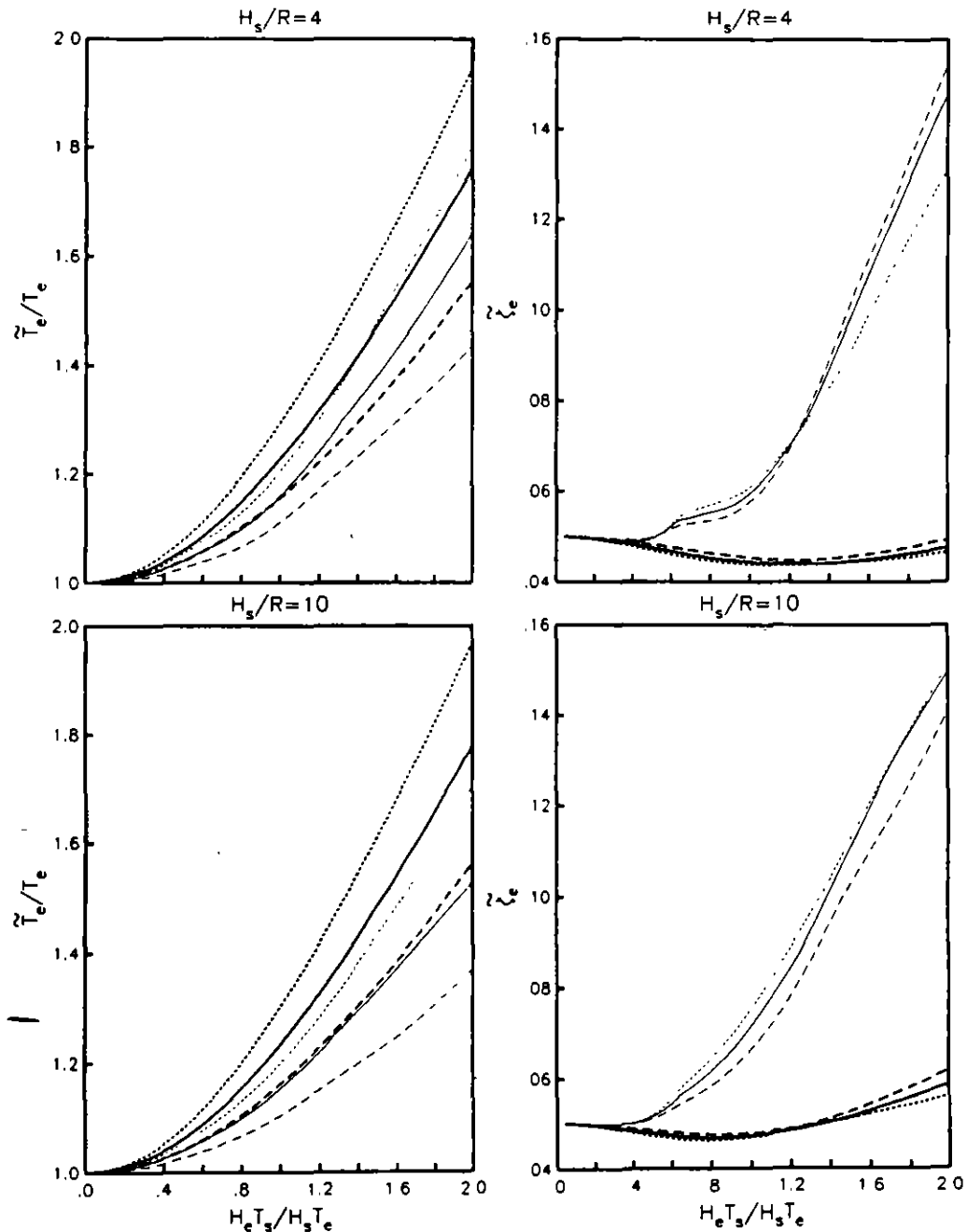
Fig. 5. Effect of the soil mass density on the effective period and damping of soil–structure systems, varying the mass density ratio as M_s/(\rho_s \pi R^2 H_s) = 0.1 (dashed line), 0.15 (solid line) and 0.2 (dotted line). Boxes correspond to H_s/R = 4 and 10, inside of which results are depicted for H_e/R = 2 (thin outline) and 5 (thick outline); \zeta_e = \zeta_s = 0.05 , \nu_s = 0.45 , D/R = 1 and E/D = 1
