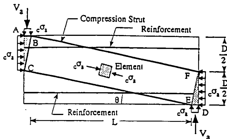
Fig. C6.2 Arch mechanism.
