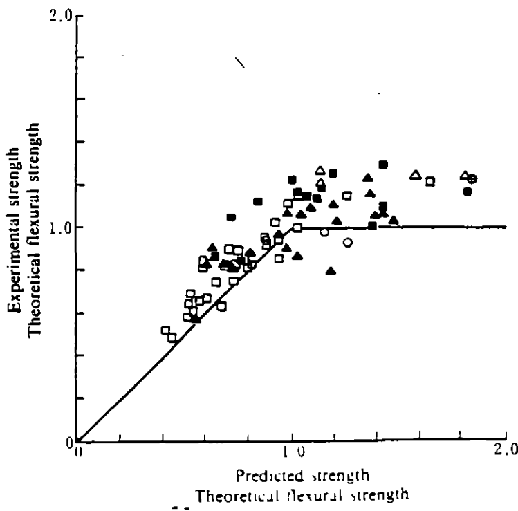
Fig. C6.17 Verification of the design equation for a non-hinge region.
