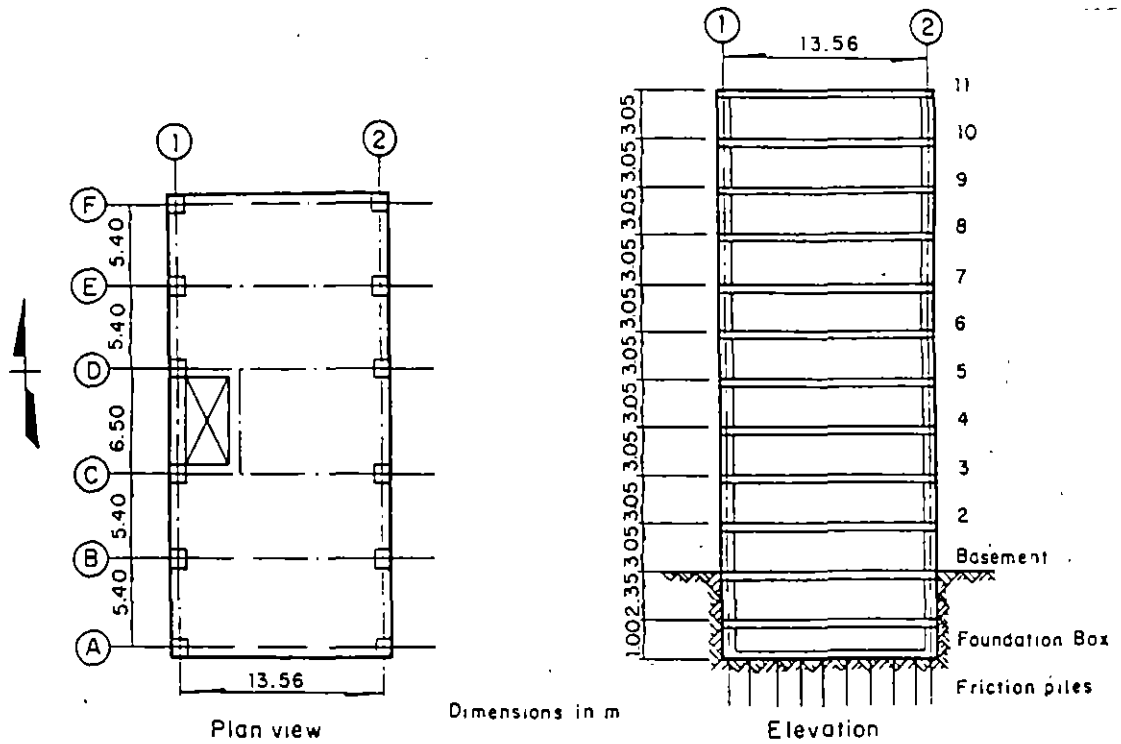
Fig. 7. Plan and elevation of the QRO Building.
