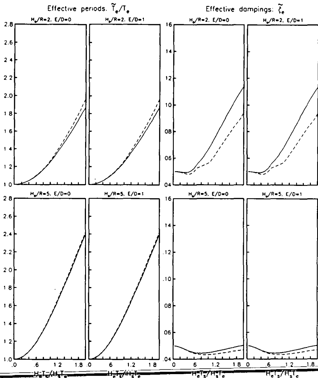
Fig. 8. Influence of the layer depth on the effective period and damping of soil-structure systems for a surface foundation with D/R = 0 . Boxes correspond to H_s/R = 2 and 5 and E/D = 0 and 1 , inside of which results are displayed for relative stratum depths H_s-tilde/R_s-tilde = 4 (dashed line) and 10 (solid line); \zeta_r = \zeta_s = 0.05 and \nu_s = 0.45 .
