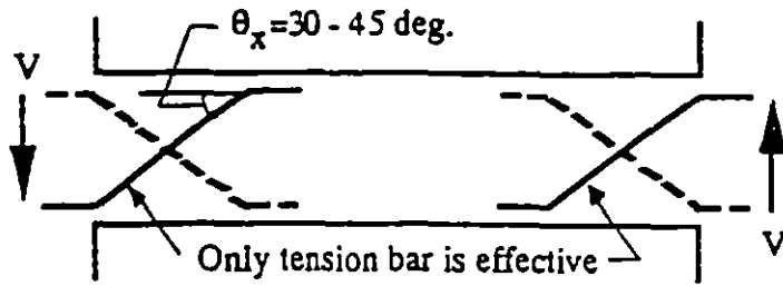
Fig. C6.14 X-shaped reinforcement in the hinge regions.
