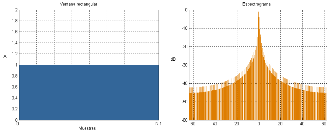
Figura 48: Ventana rectangular
