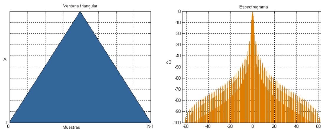
Figura 53: Ventana Triangular
