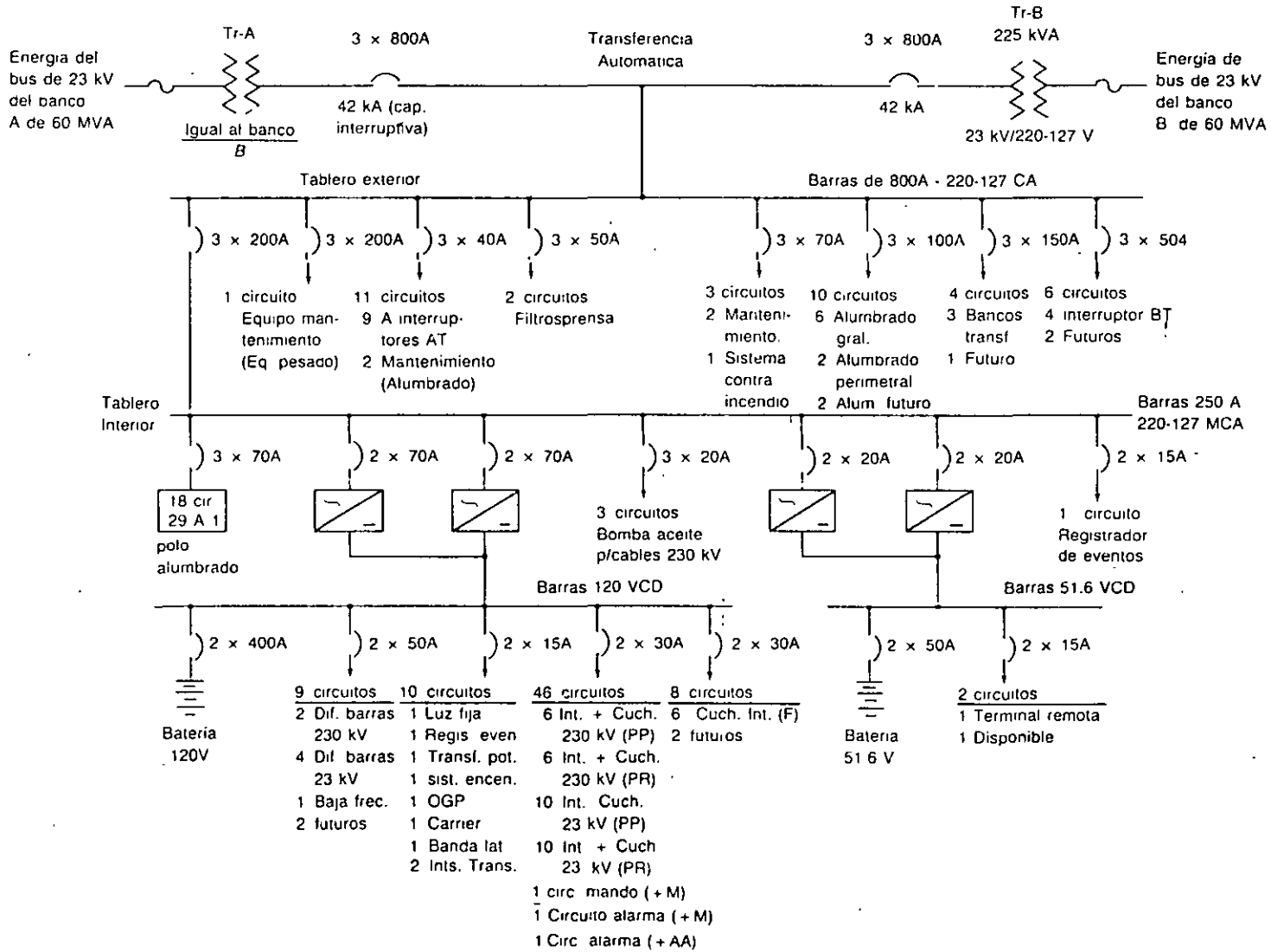
FIG. 6-1 Diagrama unifilar
