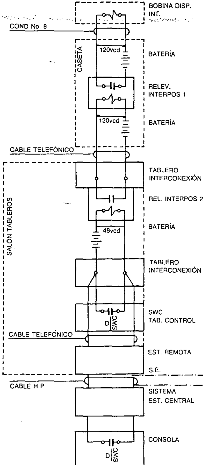
FIG. 10-4 Telecontrol interruptor 400 kV
