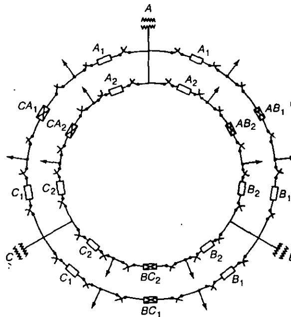
DIAGRAMA UNIFILAR
