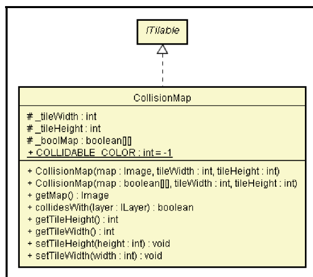
Figura 2.17: Diagrama de Clases, CollisionMap
