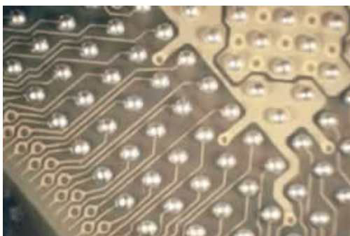
Figura III.48 Solder-ball
