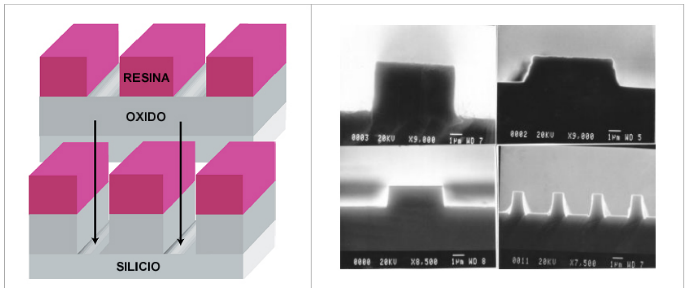
Figura III.26 Grabado seco
