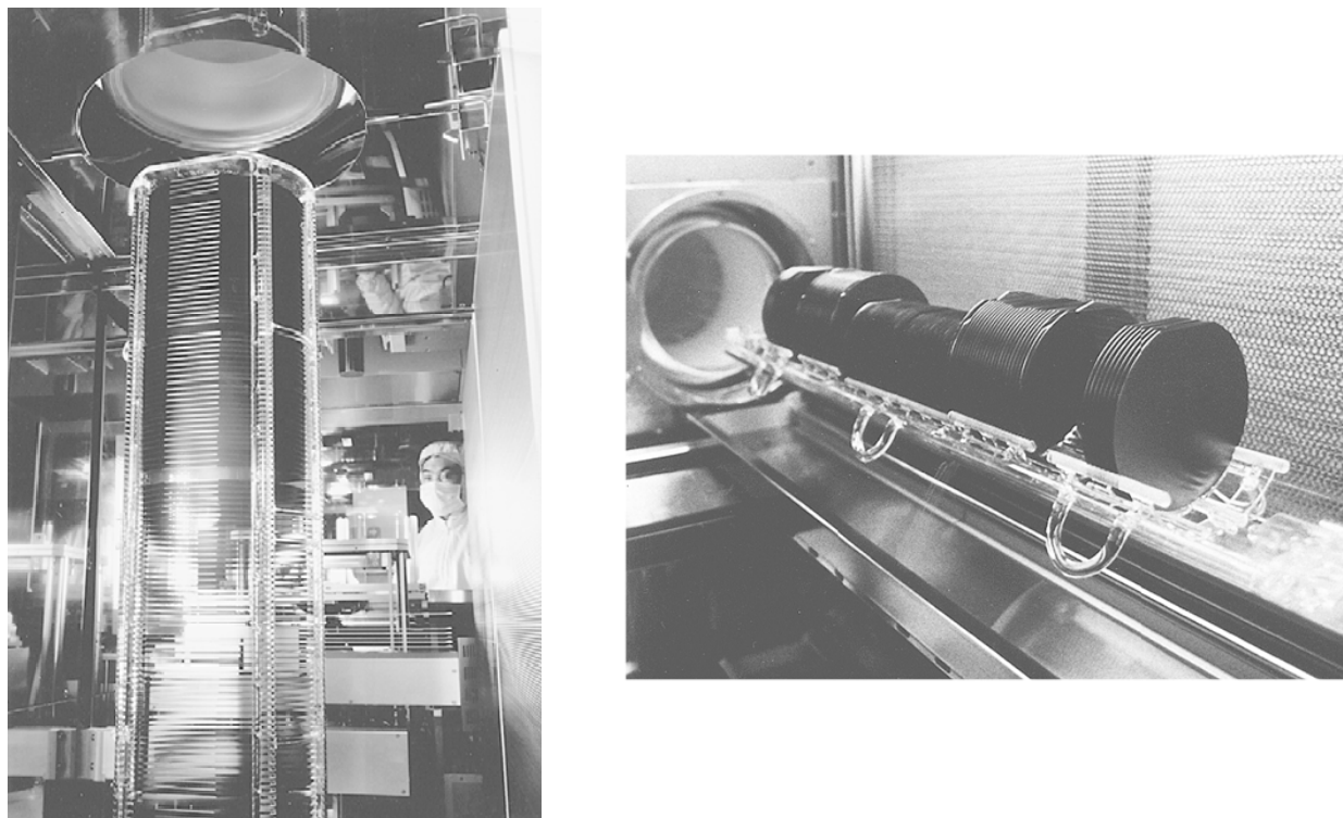
Figura III.17 Horno vertical y horizontal
