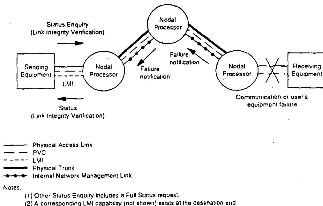
Figure 11.19 LMI environment.
