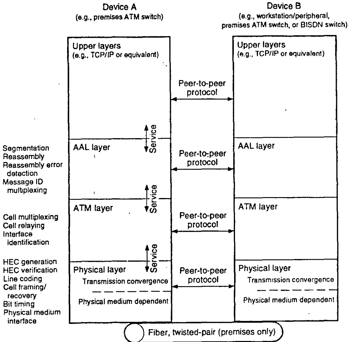
Figure 2.6 ATM protocols.
