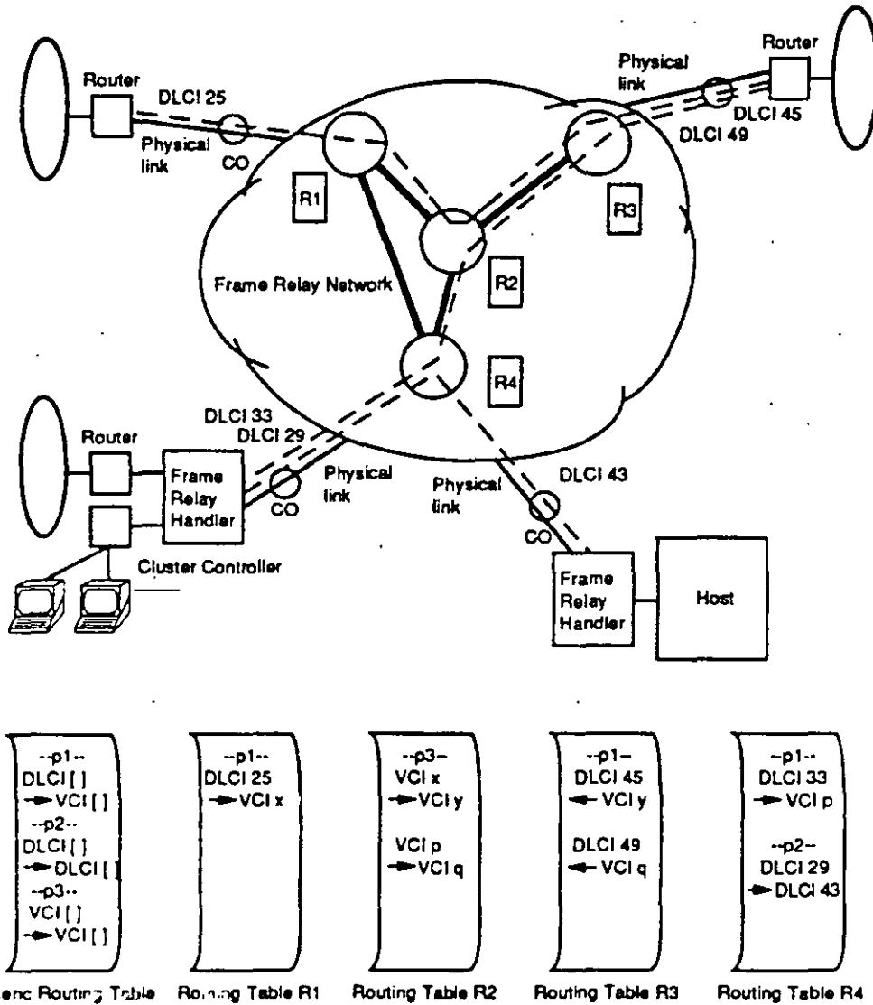
Figure 11.8 Mapping of DLCIs in a frame relay network.
