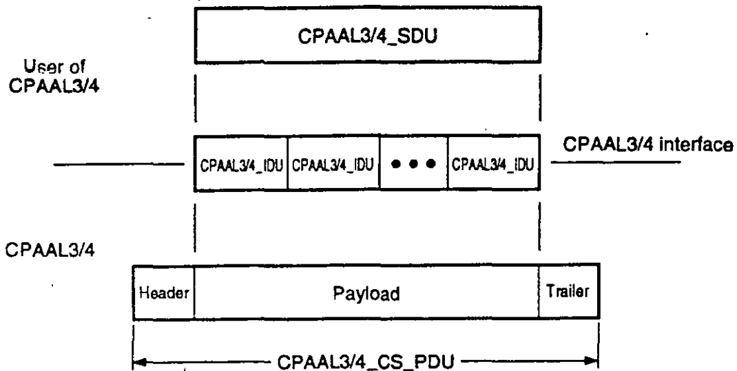
Figure 3.11 Streaming-mode service.
