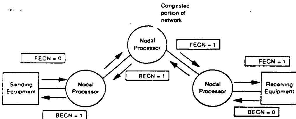
Figure 11.18 FECN and BECN action.
