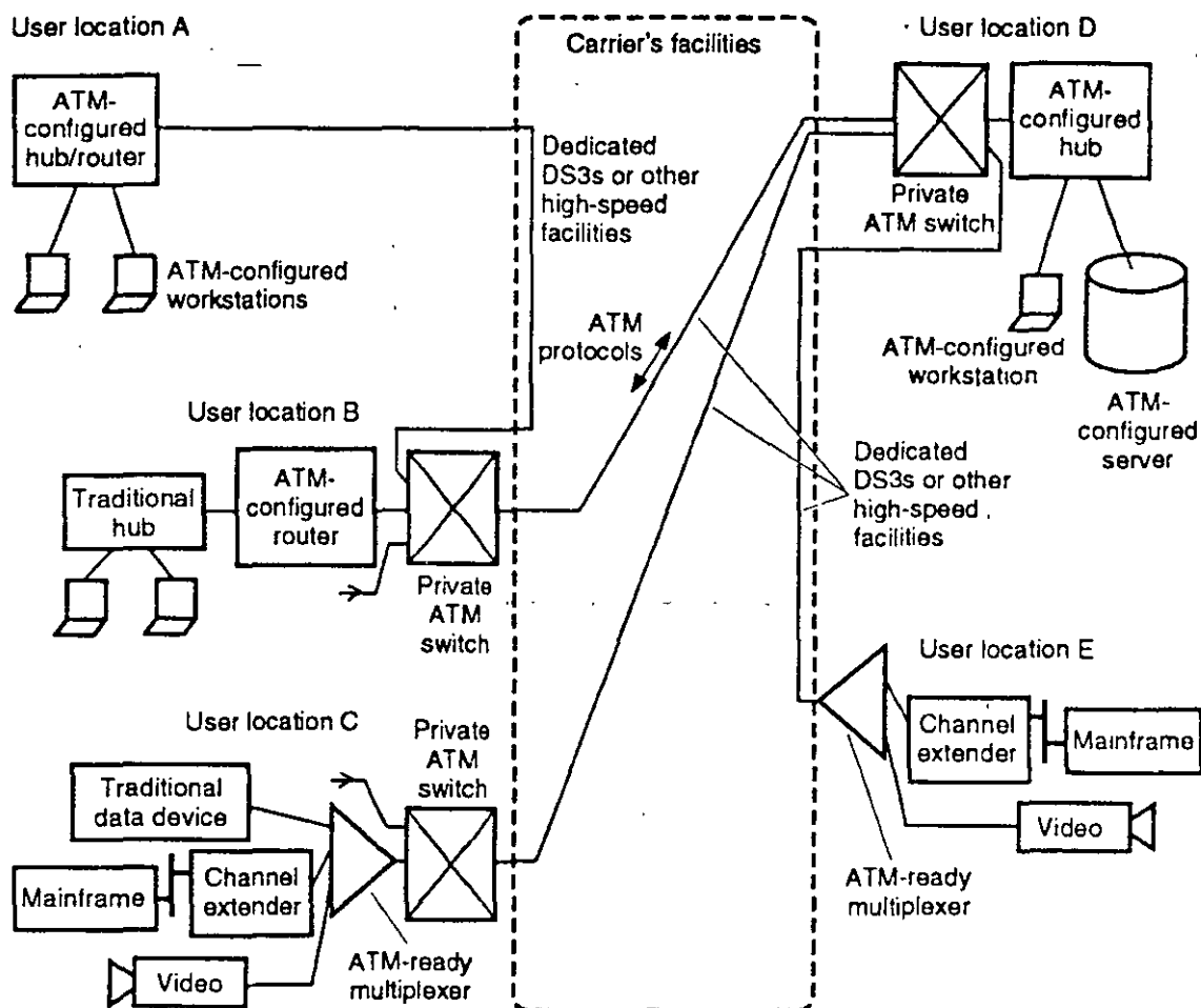
Figure 1.19 CRS to support enterprise networking in WAN applications (private network).
