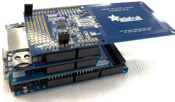
Fig. 4.11 Arduino Mega ADK + Arduino Wi-Fi Shield + Data Logger + PN532 RFID/NFC
