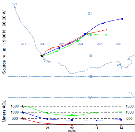
NOAA HYSPLIT MODEL Backward trajectories ending at 1200 UTC 06 Jun 15 GDAS Meteorological Data
