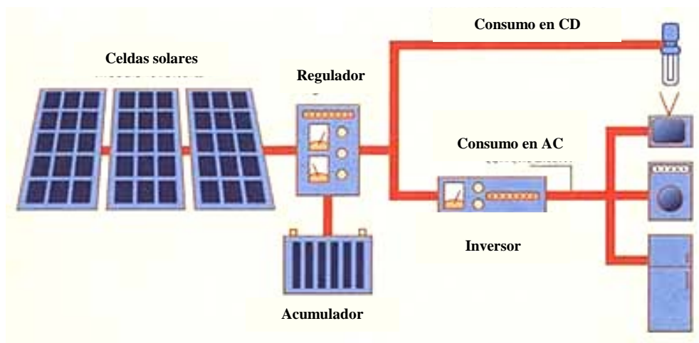
Figura 2.5: Panel solar. [123]
