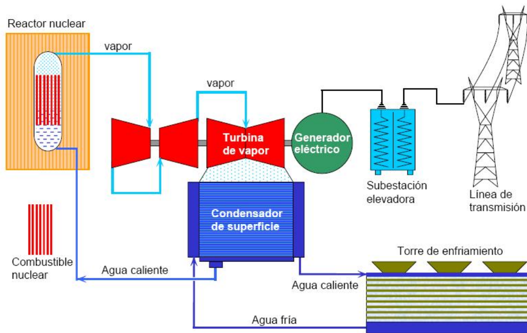
Figura 2.2: Central Nuclear. [10]
