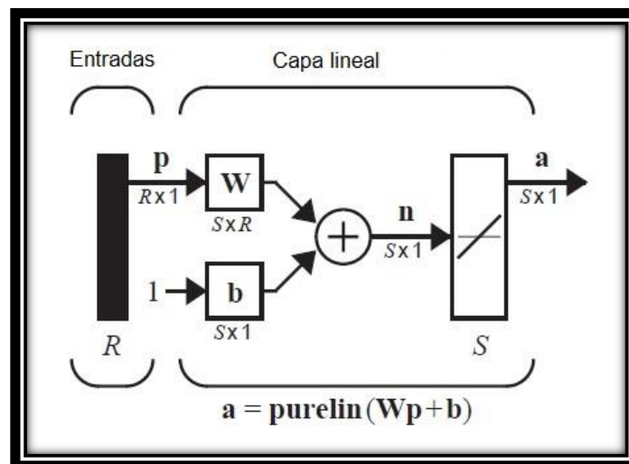
Figura 2.9 Red ADALINE
