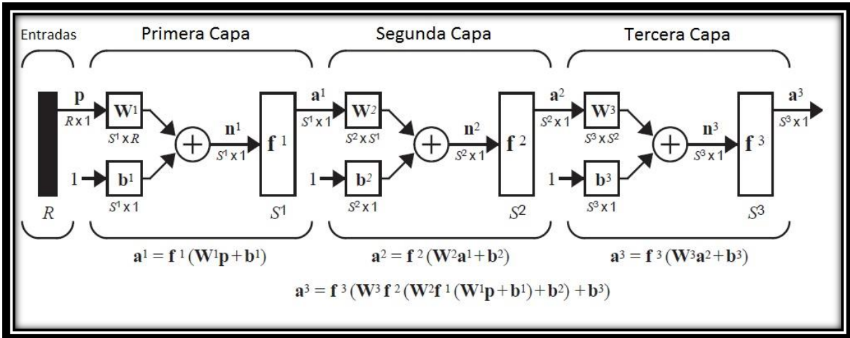
Figura 2.10 Red Multicapa
