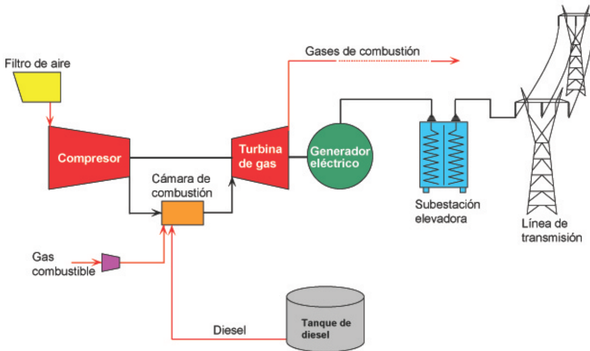
Figura I.3 Central turbogás
