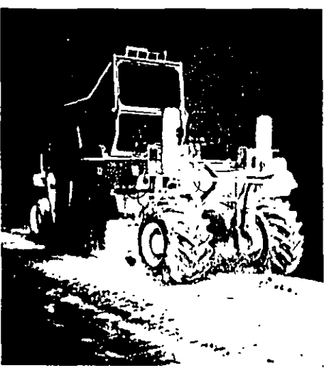
Wirtgen cold recycling: the existing road materials are reused to produce a strong foundation course.
