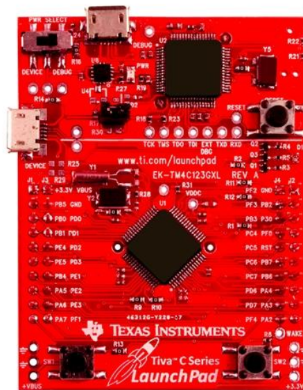
Figura 3.3. Vista frontal de tarjeta TM4C123G LaunchPad [73]
