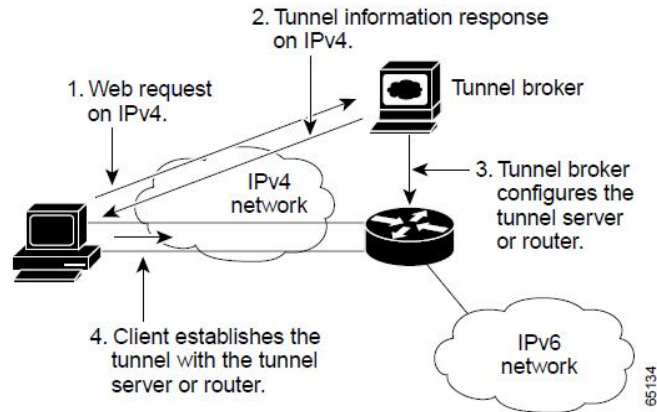
Figura 6.9 Túnel Broker.
