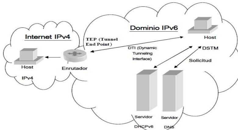
Figura 6.4 Arquitectura Dual-Stack.
