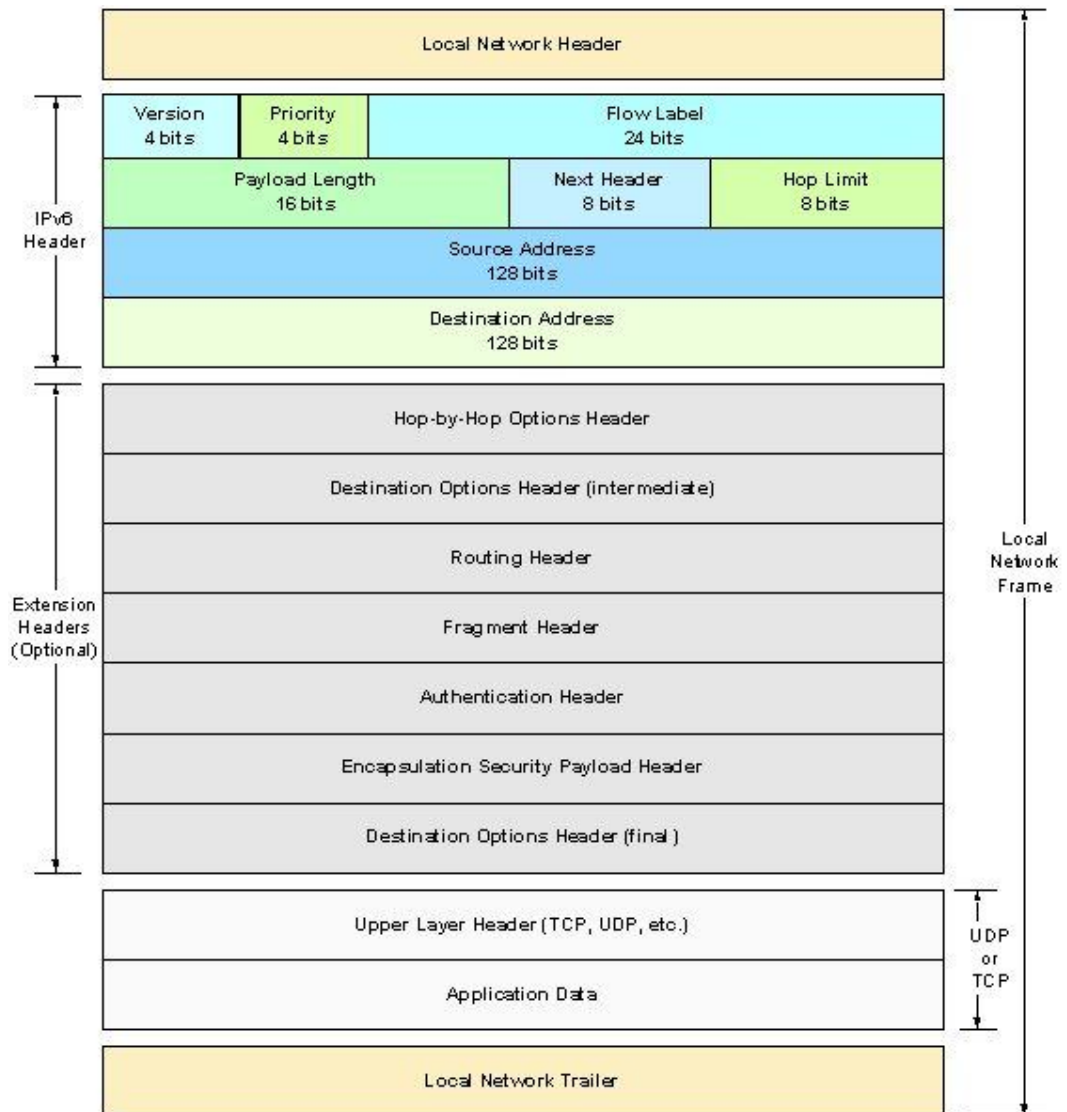
Figura 4.10 Extension Header.
