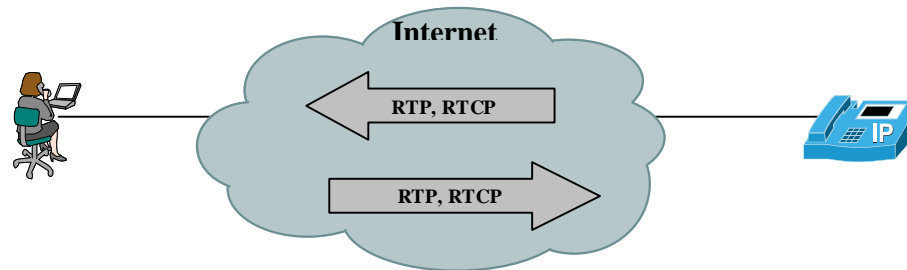
Figura 3.11 Flujo RTP/RTCP.
