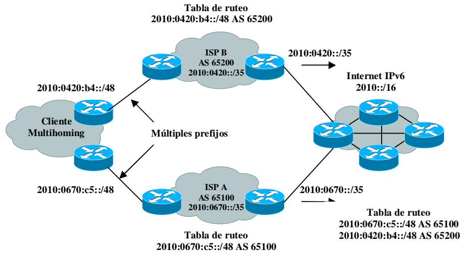
Figura 4.4 Multihoming.
