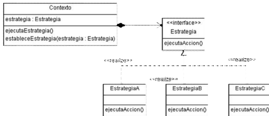
FIGURA IV.10 - STRATEGY PATTERN
