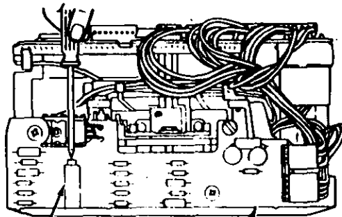
Variable Resistor
