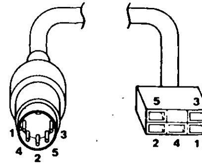
Figure 2. Continuity Check
