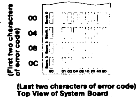
Figure 2. System Board
