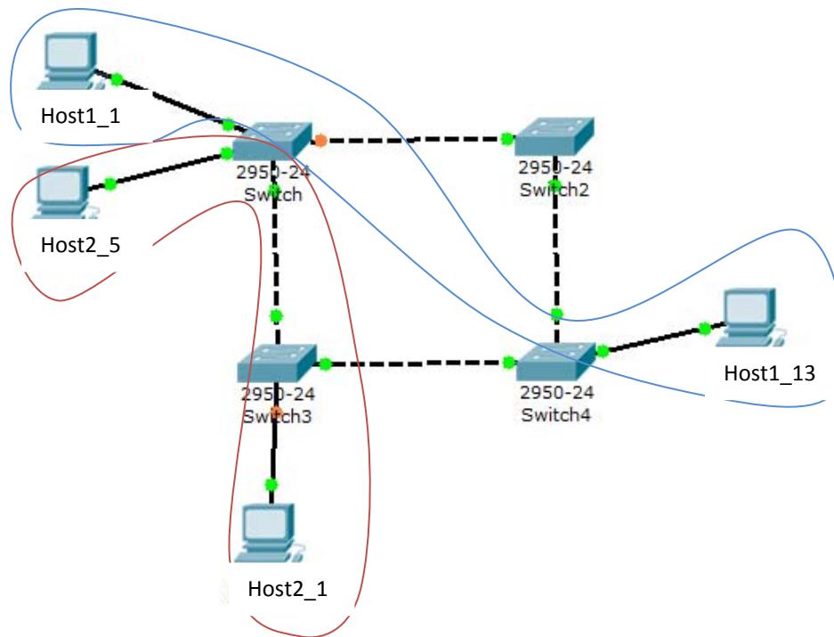
Figura 2.5 - VLANs Troncales
