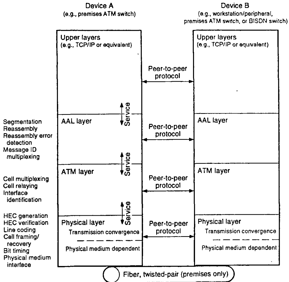
Figure 2.6 ATM protocols.
