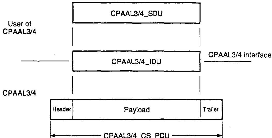
Figure 3.10 Message-mode service.
